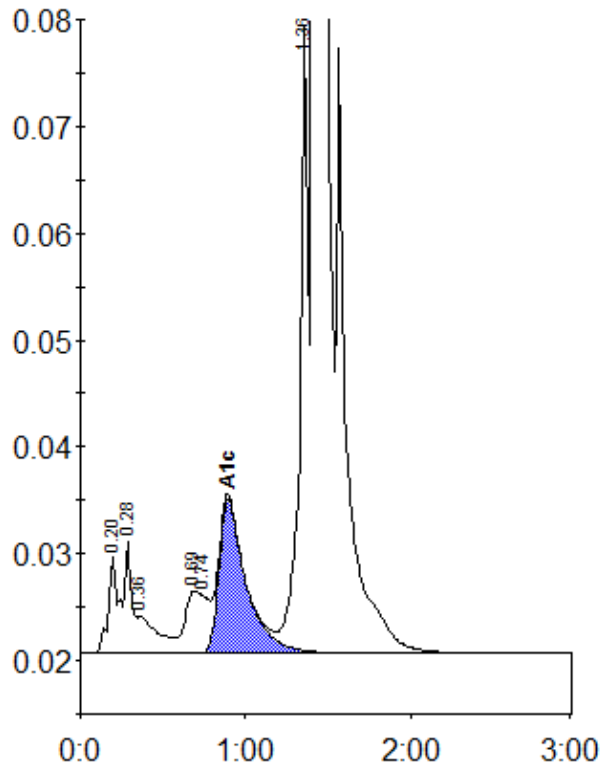
Peak table - ID: 10436186
